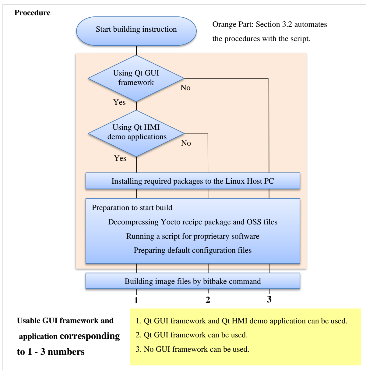
Figure 2. Building Outline
