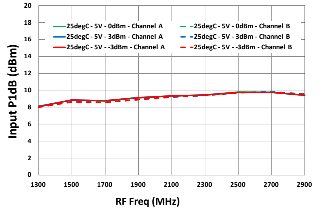
IP1dB vs. LO Power [IP1dB MXR , LS injection]
