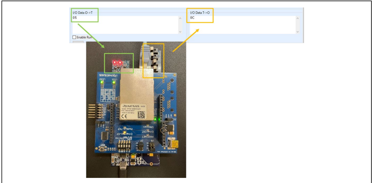
図 3-43 Remote-IO (LED/Switch)制御 [EtherNet/IP]
