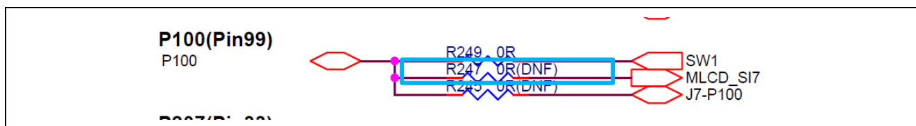
Figure 4-1 Schematic diagram of Evaluation Kit RE01 1500KB main board (R247 part)
