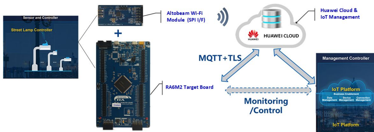
Figure: Huawei Cloud Smart Street Lighting Solution
