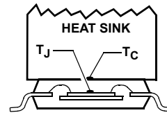
FIGURE 4B. NON-ENHANCED PACKAGE TOP (HEAT SINK ON TOP)
