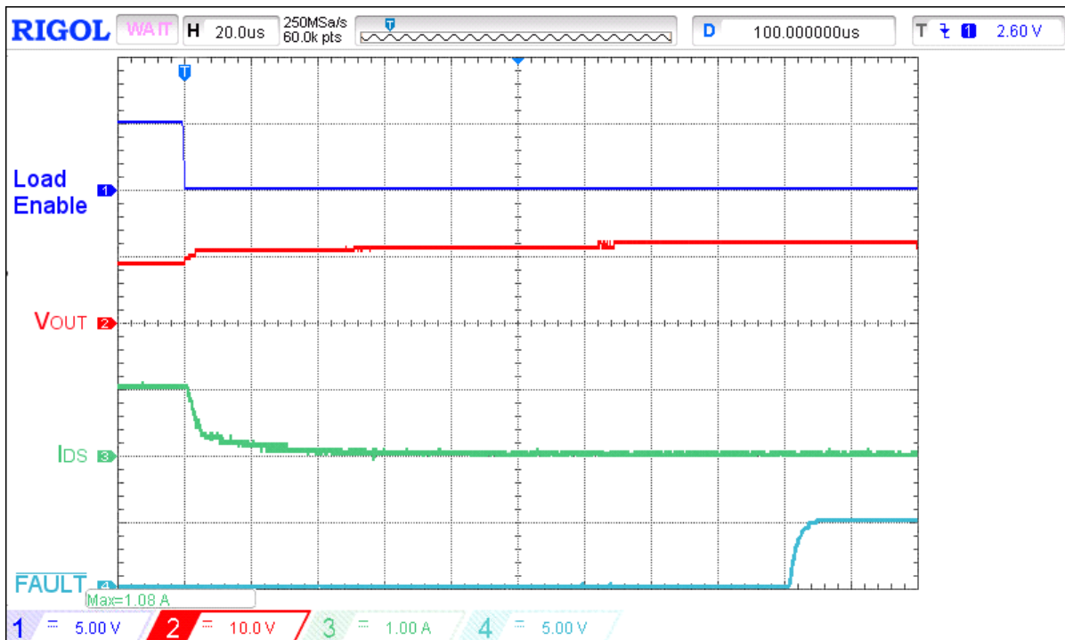
Figure 28. Typical FAULT de-assertion waveform for V_{IN} = 12\text{ V} , C_{LOAD} = 10\text{ }\mu\text{F} , I_{ACL} = 1\text{ A} , R_{SET} = 91\text{ k}\Omega , switch out 9\text{ }\Omega load
