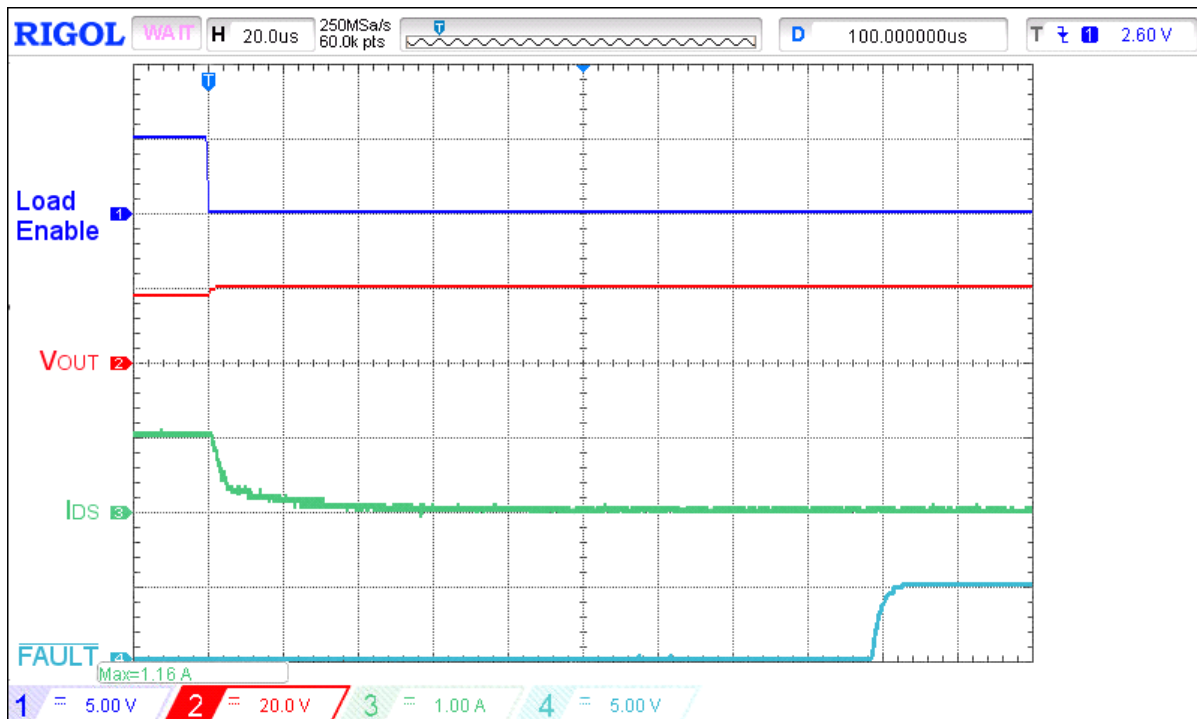
Figure 30. Typical FAULT de-assertion waveform for V_{IN} = 20\text{ V} , C_{LOAD} = 10\text{ }\mu\text{F} , I_{ACL} = 1\text{ A} , R_{SET} = 91\text{ k}\Omega , switch out 15\text{ }\Omega load
