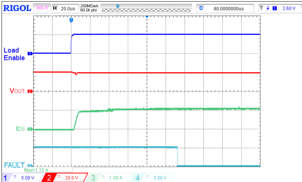
Figure 29. Typical FAULT assertion waveform for V_{IN} = 20\text{ V} , C_{LOAD} = 10\text{ }\mu\text{F} , I_{ACL} = 1\text{ A} , R_{SET} = 91\text{ k}\Omega , switch on 15\text{ }\Omega load
