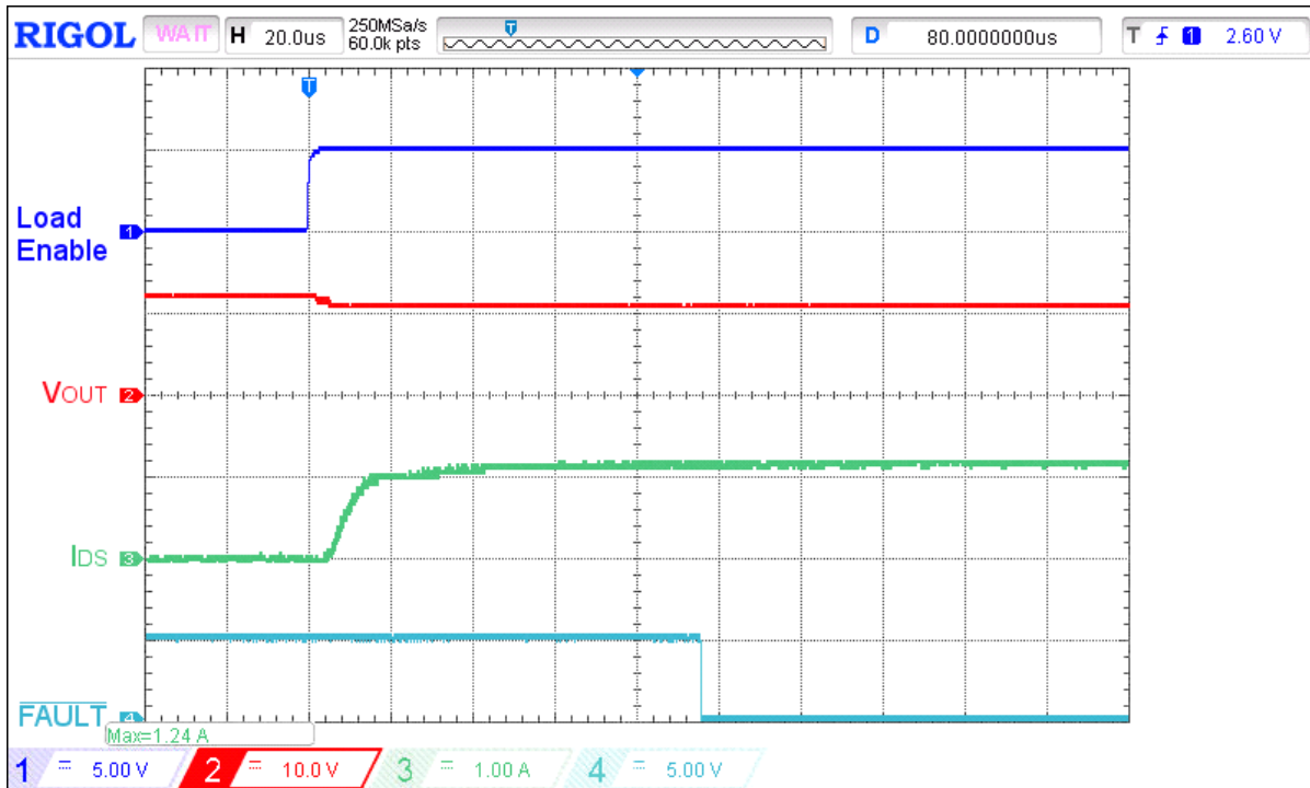
Figure 27. Typical FAULT assertion waveform for V_{IN} = 12\text{ V} , C_{LOAD} = 10\text{ }\mu\text{F} , I_{ACL} = 1\text{ A} , R_{SET} = 91\text{ k}\Omega , switch on 9\text{ }\Omega load
