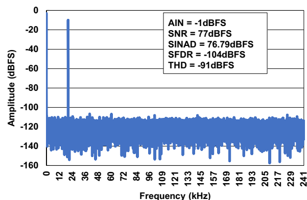
Figure 2. FFT - 20.3kHz
