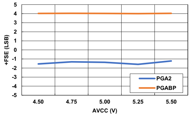
Figure 44. +Full-Scale Error vs AV_{CC}
