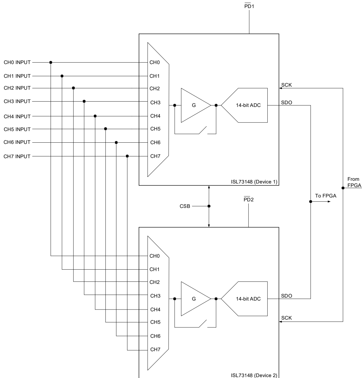
Figure 126. ISL73148SEH Cold Sparring Example Circuit
