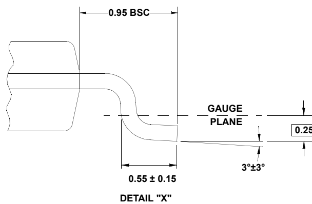
DETAIL "X"
