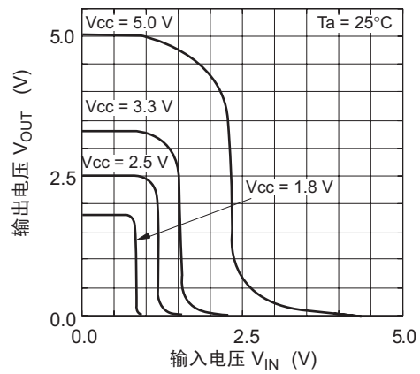
(HD74LV1GU04A)
