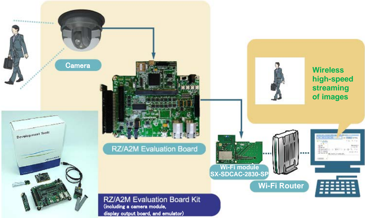
Figure 1 RZ/A2M SDIO Wi-Fi Package Sample Application Image
