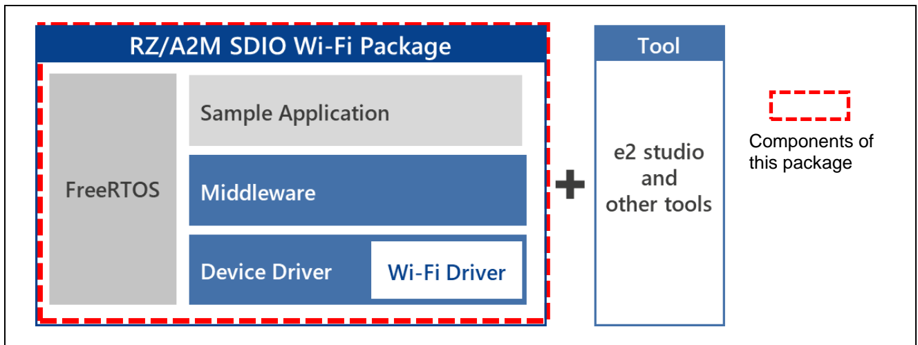
Figure 2 Software Structure of the RZ/A2M SDIO Wi-Fi Package
