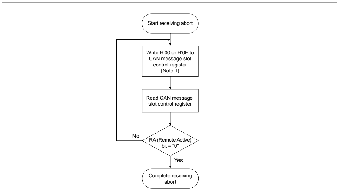
Figure 2. Operation flow when canceling remote frame receiving
