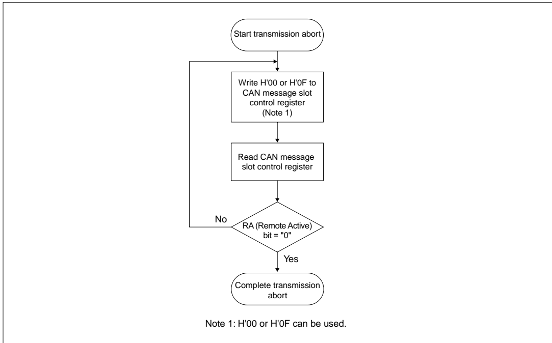
Figure 1. Operation flow when aborting remote frame transmission
