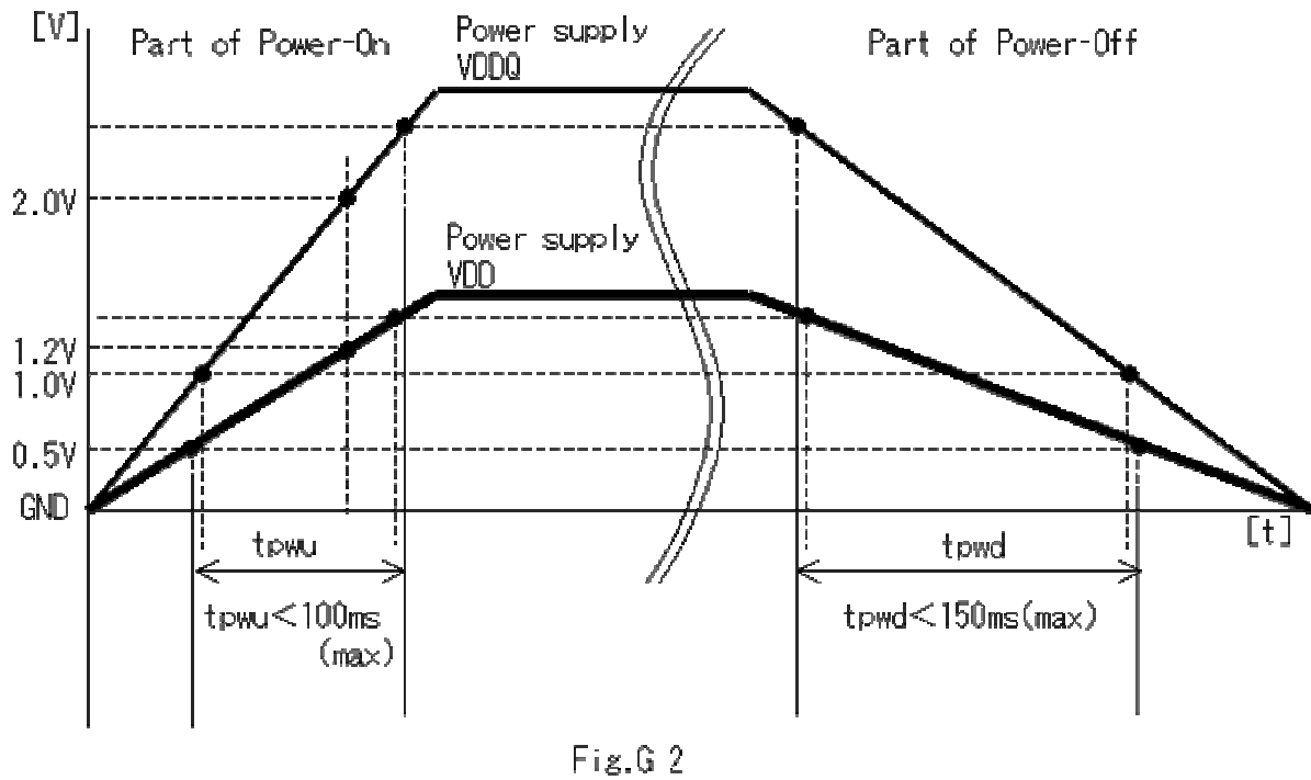
Fig.G Power-On and Power-Off procedure
