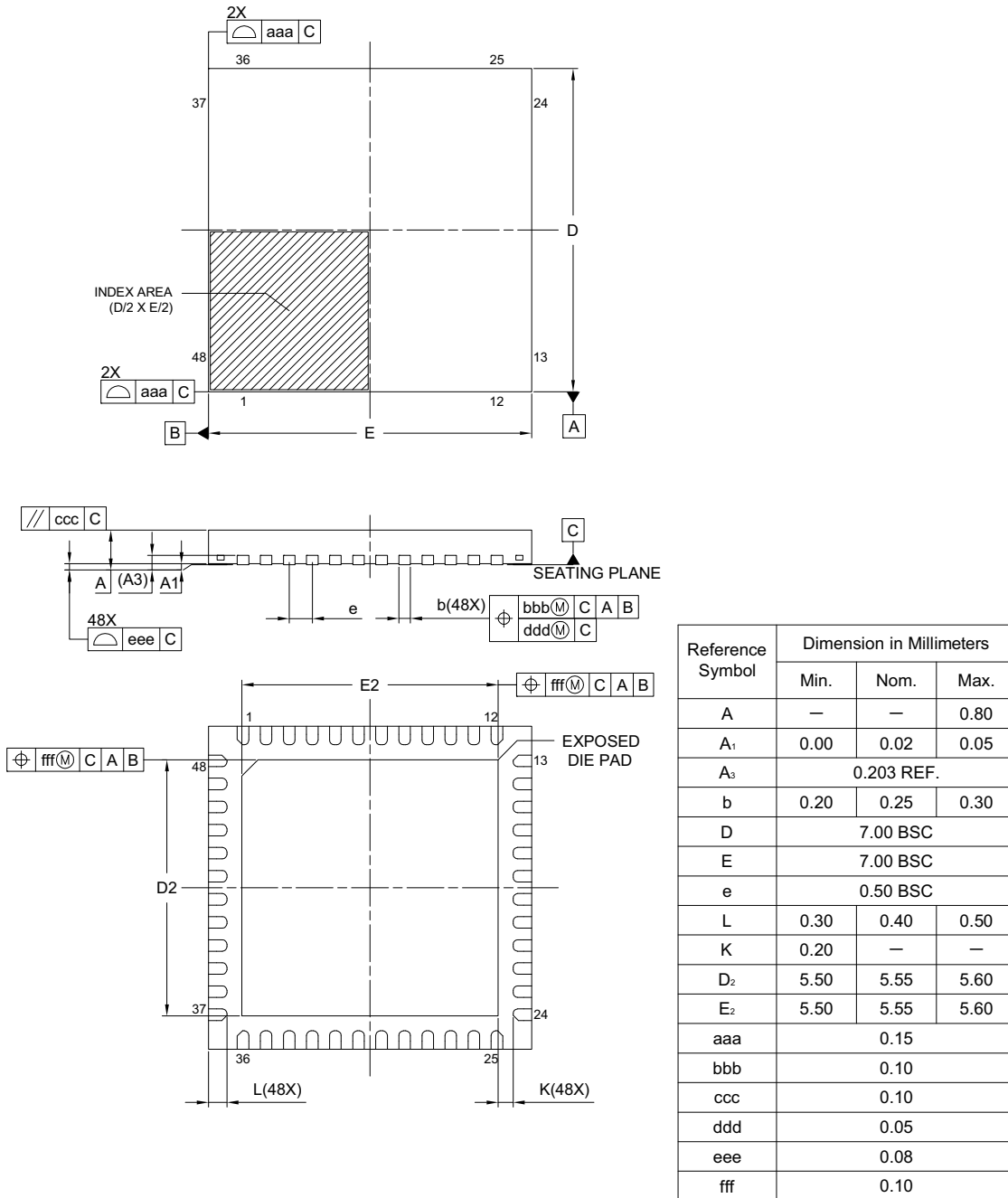
Figure 2. 48-Pin HWQFN (PWQN0048KE-A)
