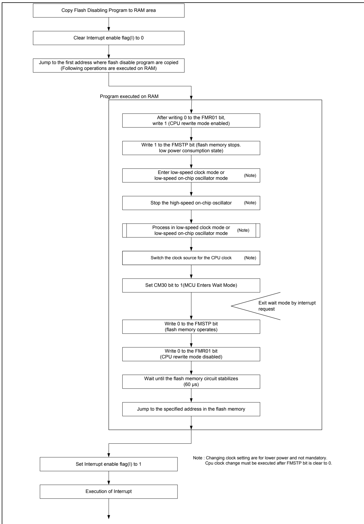
Fig 1 Flow chart of software workaround
