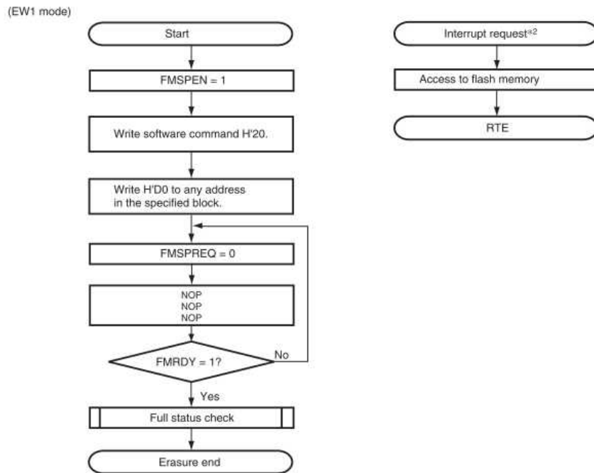
Figure 7.15 Flowchart When Erase-Suspend Function is Used EW1 mode
