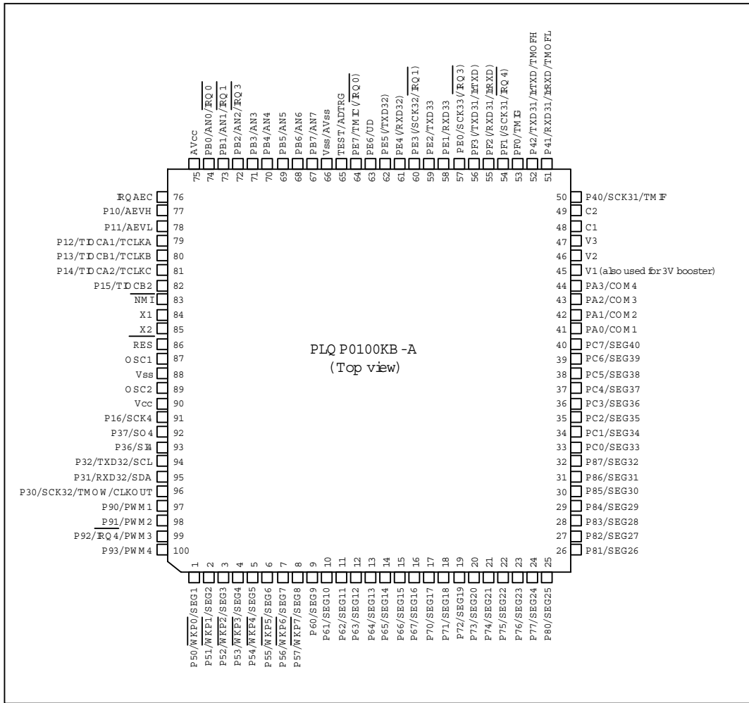
Figure 1. 2 Pin Assignment of H8/38099 Group (PLQ P0100KB -A)
