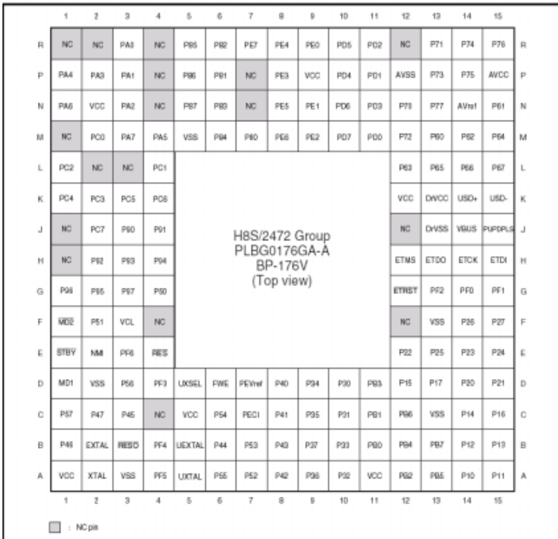
Figure 1.2 Pin Assignments (H8S/2472 Group)
