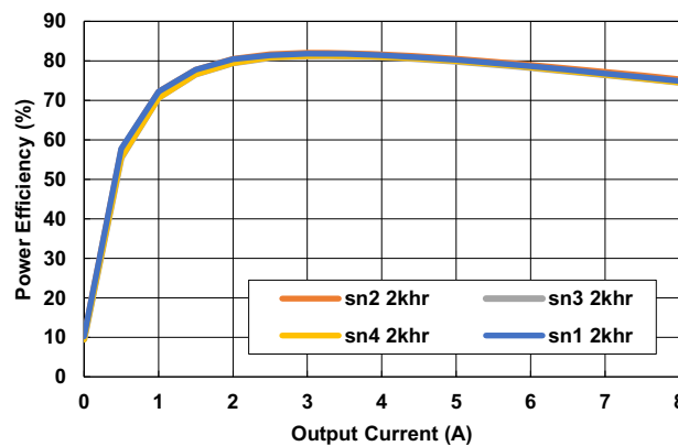
Figure 5. Comparison of All Four Devices Post High Power Stress Efficiency Curves
