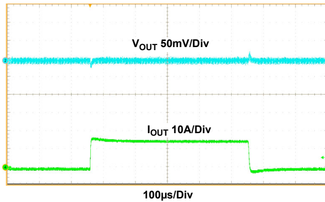
Figure 18. Transient Response, V_{IN} = 12V , V_{OUT} = 1.2V , 0A to 15A to 0A, 5A/μs Step Load, C_{OUT} = 7 \times 47\mu F Ceramic + 2 \times 470\mu F Polymer Capacitor
