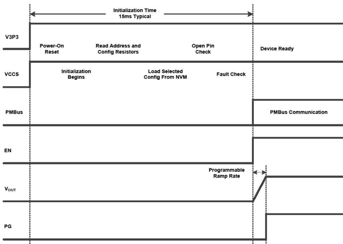
Figure 34. Simplified PMBus Initialization Timing Diagram
