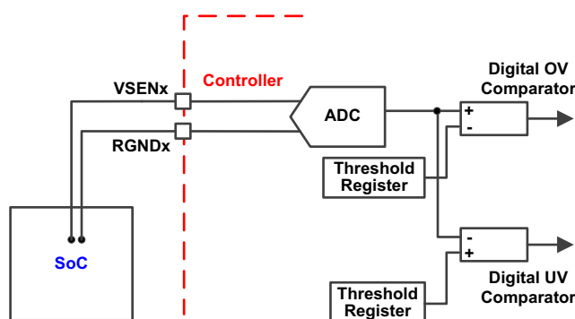
Figure 36. OV/UV Comparators
