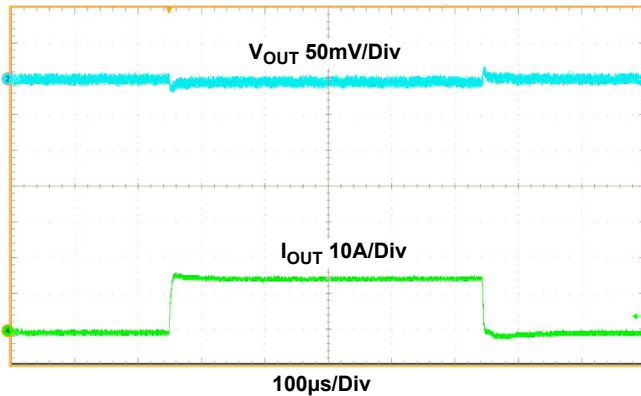
Figure 20. Transient Response, V_{OUT} = 3.3V , 0A to 15A, 5A/μs Step Load, C_{OUT} = 15 \times 47\mu F Ceramic + 2 \times 470\mu F Polymer Capacitor
