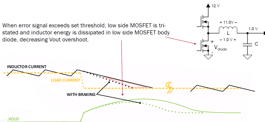
Figure 35. Body Diode Braking Operation
