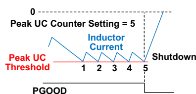
Figure 38. Peak UC Operation
