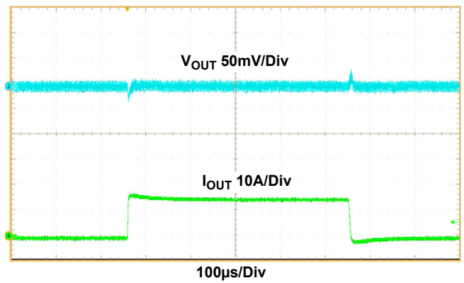
Figure 19. Transient Response, V_{OUT} = 1.8V , 0A to 15A, 5A/μs Step Load, C_{OUT} = 7 \times 47\mu F Ceramic + 2 \times 470\mu F Polymer Capacitor
