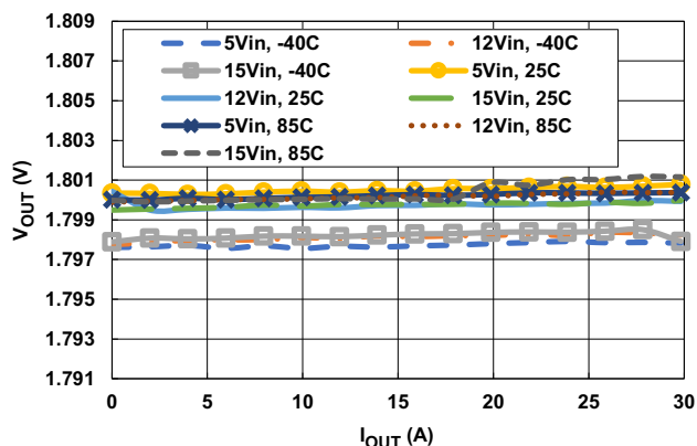
Figure 11. Load Regulation over V_{IN} and Temperature V_{OUT} = 1.8V , V_{IN} = 5V, 12V, 15V , Temperature = -40, 25, 85^\circ C
