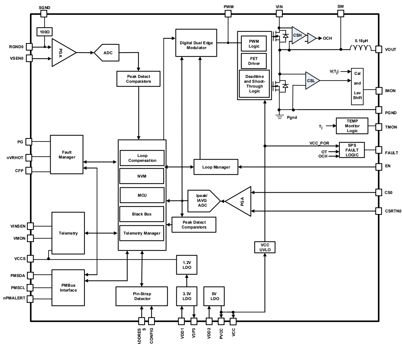
Figure 2. Block Diagram
