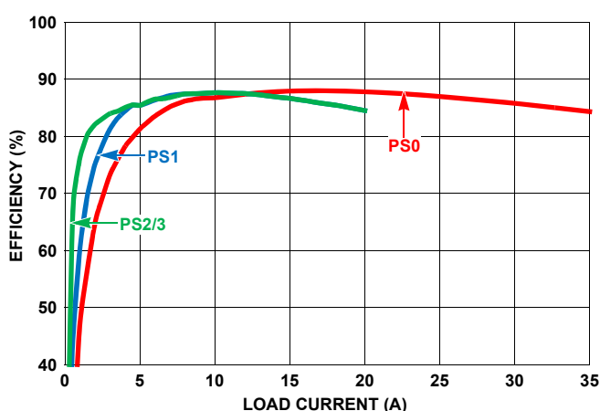
FIGURE 2. VR B EFFICIENCY vs LOAD
