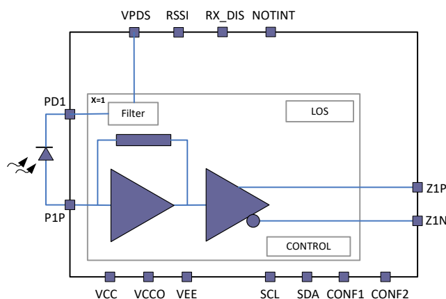
Figure 1: Device diagram
