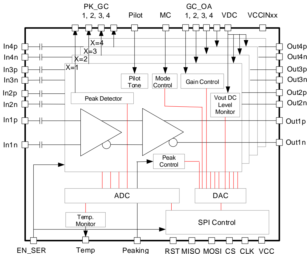
Figure 1. Block Diagram
