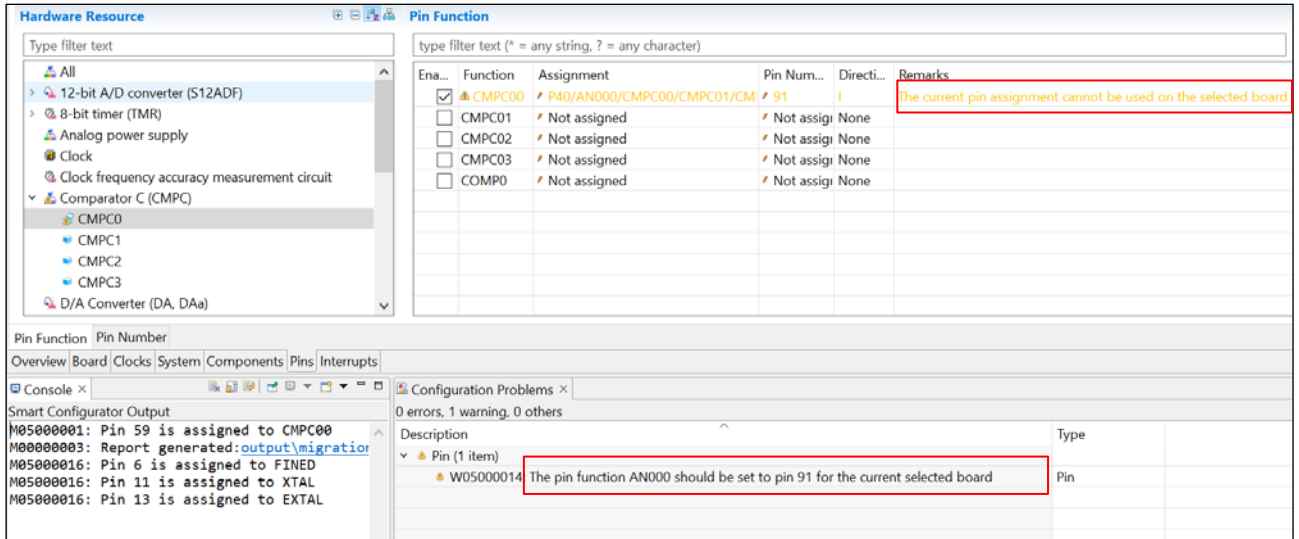
Figure 3-2 Pin warning message in Smart Configurator RX 2.14.0 or before
