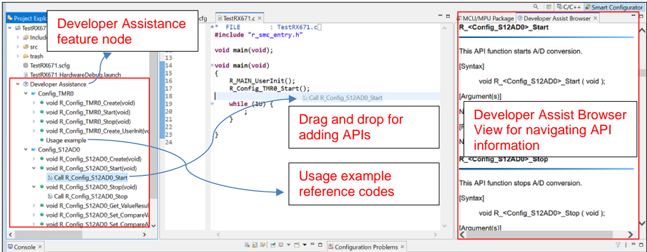
Figure 2-2 Developer Assistance feature for Code Generator components
