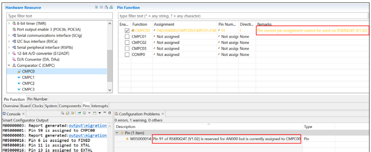
Figure 3-3 Pin warning message in Smart Configurator RX 2.15.0 or later
