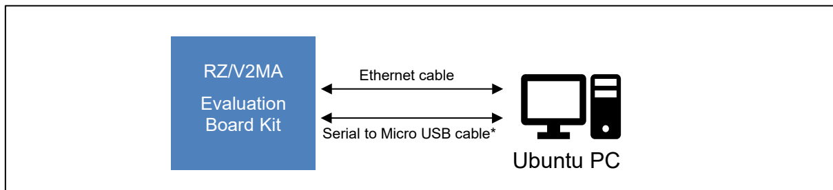
Figure 3-1 Hardware Configuration
