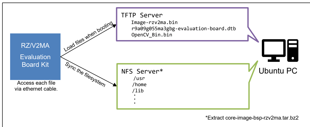
Figure 3-2 Network Booting Overview
