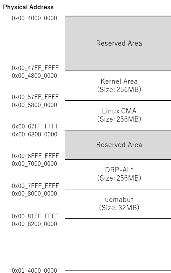
Figure 2. Memory map
