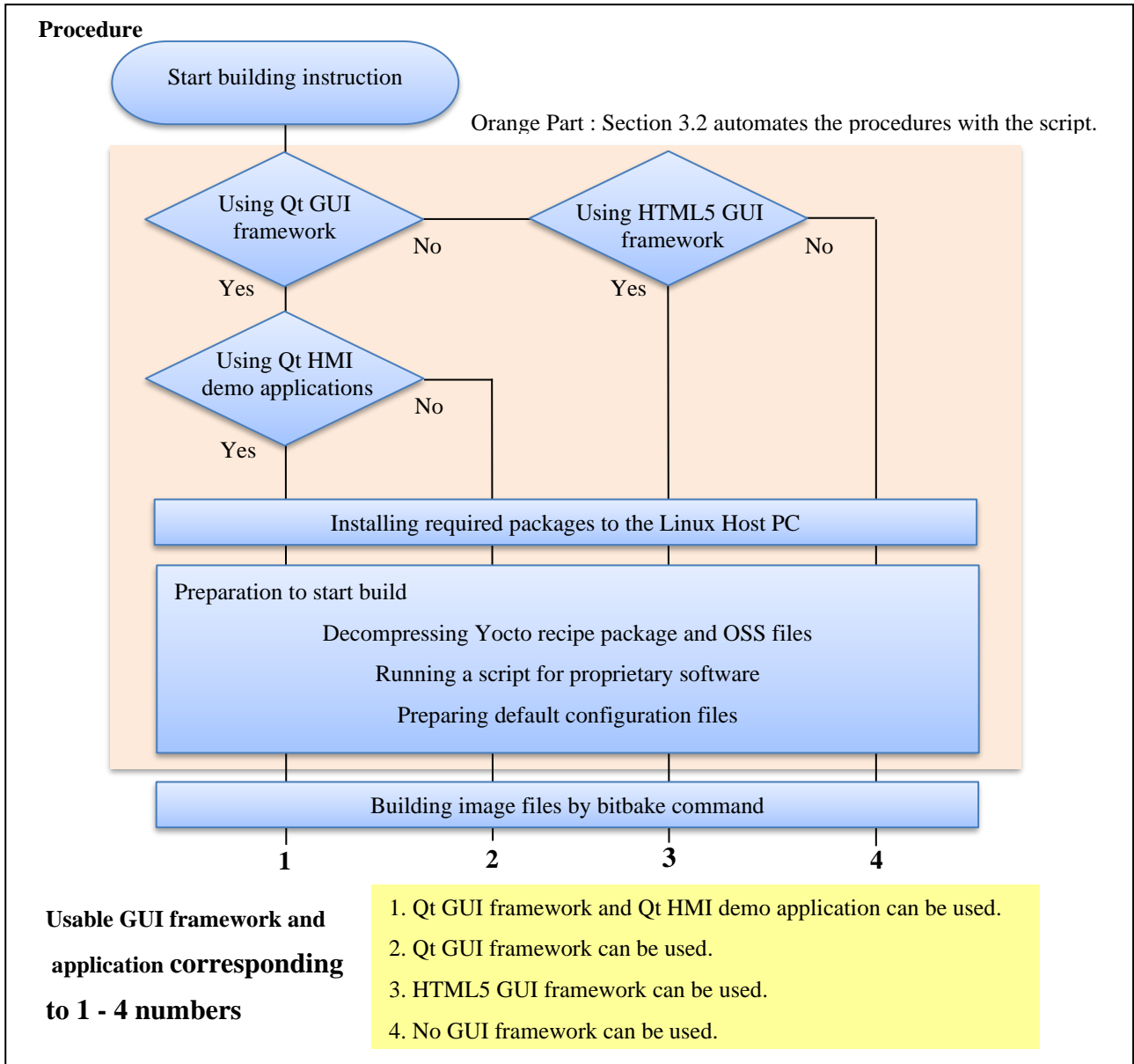
Figure 2. Building Outline
