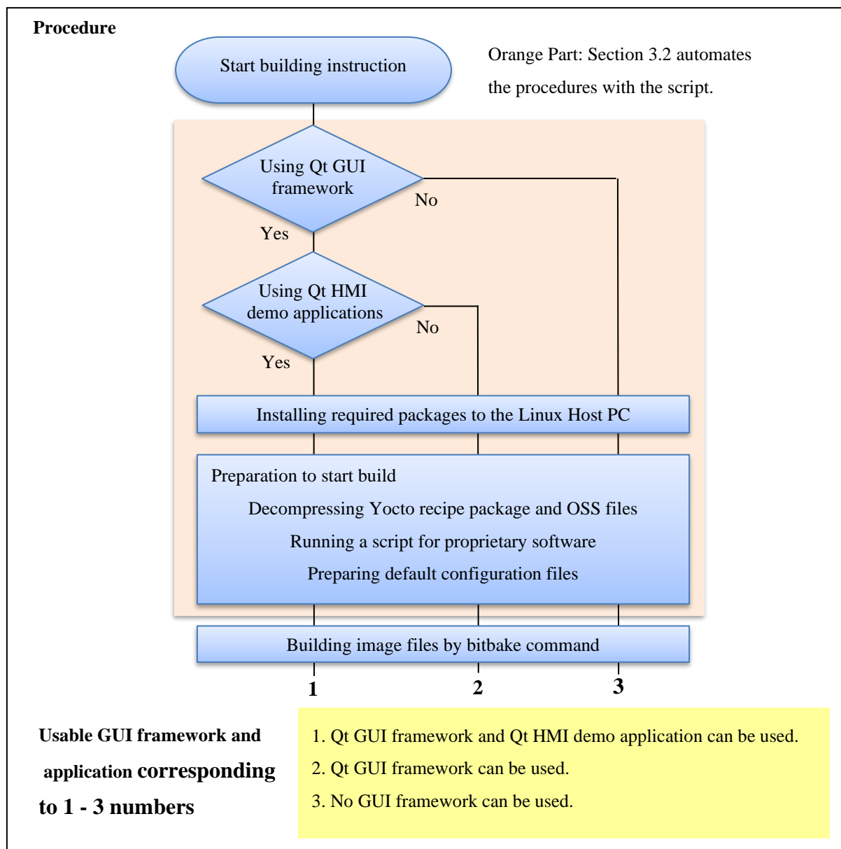
Figure 2. Building Outline
