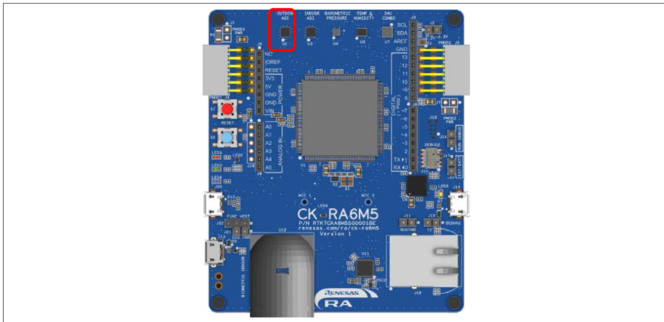
Figure 2. CK-RA6M5 Board showing Outdoor Air Quality Sensor U2 Location
