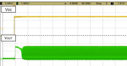
Oscillation start up waveform on recommendable circuit condition MODEL: CSTCE8M00G55-R0 with R5F213NCTDBX(CM11=0)
