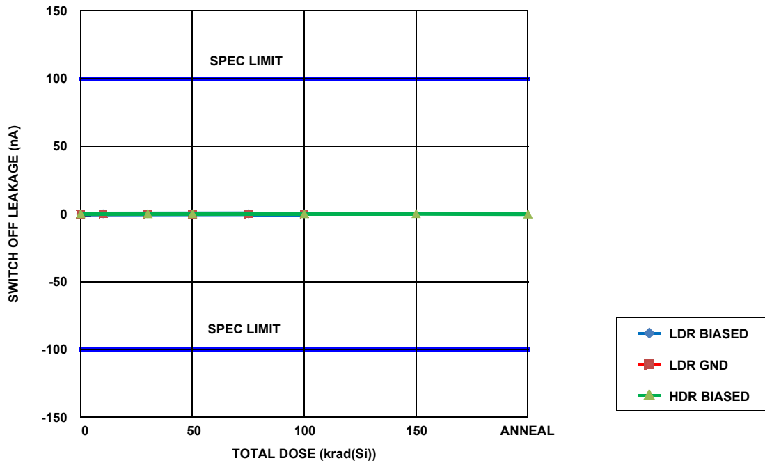
FIGURE 14. ISL7x840SEH switch OFF leakage ( I_{S(OFF)} ) into the source of an unselected channel, average of all 16 channels, supply voltage \pm 15V , input voltage +11.5V , as a function of total dose irradiation at HDR for the biased (per Figure 2) case and at LDR for the unbiased (all pins grounded) and the biased (per Figure 2) cases. The LDR was 0.0089\text{rad(Si)/s} and the HDR was 69.72\text{rad(Si)/s} . Sample size for each of the three cells was 4. The post-irradiation SMD limits are -100\text{nA} to 100\text{nA} .
