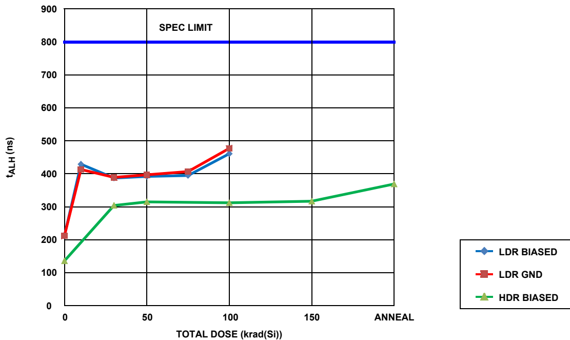
FIGURE 33. ISL7x840SEH address to output access time, LOW-to-HIGH, supply voltage ±12V, as a function of total dose irradiation at HDR for the biased (per Figure 2) case and at LDR for the unbiased (all pins grounded) and the biased (per Figure 2) cases. The LDR was 0.0089rad(Si)/s and the HDR was 69.72rad(Si)/s. Sample size for each of the three cells was 4. The post-irradiation SMD limit is 800ns maximum.
