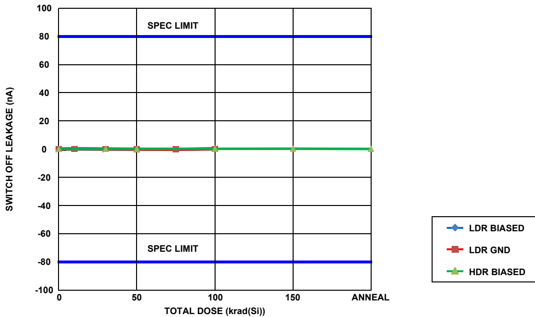
FIGURE 26. ISL7x840SEH switch OFF leakage ( I_{D(OFF)} ) into the drain with the part disabled, supply voltage \pm 15V , output voltage +10V , input voltage -10V , as a function of total dose irradiation at HDR for the biased (per Figure 2) case and at LDR for the unbiased (all pins grounded) and the biased (per Figure 2) cases. The LDR was 0.0089\text{rad(Si)/s} and the HDR was 69.72\text{rad(Si)/s} . Sample size for each of the three cells was 4. The post-irradiation SMD limits are -80\text{nA} to +80\text{nA} .
