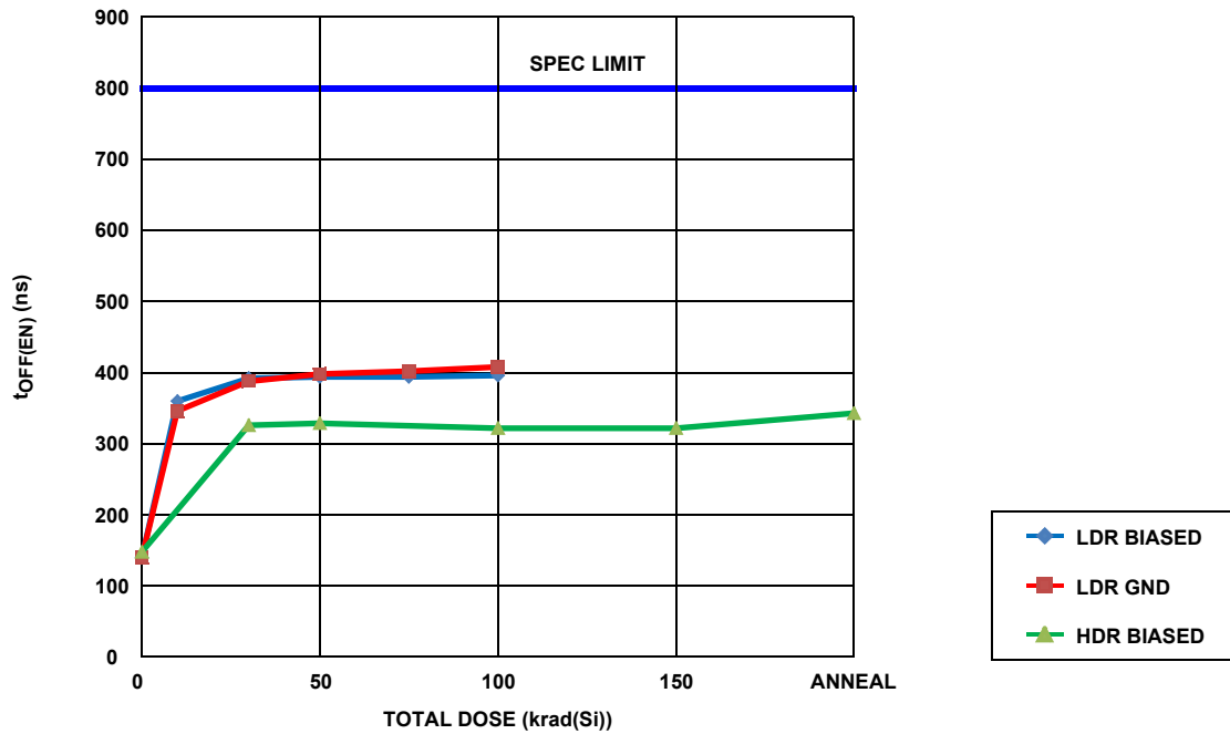
FIGURE 32. ISL7x840SEH enable to output OFF delay, supply voltage ±15V, as a function of total dose irradiation at HDR for the biased (per Figure 2) case and at LDR for the unbiased (all pins grounded) and the biased (per Figure 2) cases. The LDR was 0.0089rad(Si)/s and the HDR was 69.72rad(Si)/s. Sample size for each of the three cells was 4. The post-irradiation SMD limit is 800ns maximum.
