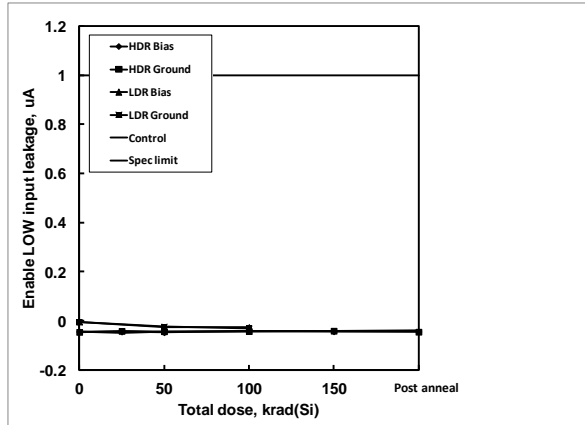
Figure 2: ISL75051SEH enable LOW input current as a function of biased and grounded high and low dose rate irradiation and subsequent high temperature accelerated post-high dose rate aging at 100^{\circ}\text{C} . The dose rate was 80 \text{ rad}(\text{Si})/\text{s} . Sample size was 6 for the high dose rate cells and 4 for the low dose rate cells, and three control units were used for the high dose rate test. The specification limits are -0.100\mu\text{A} - +1.000\mu\text{A} .
