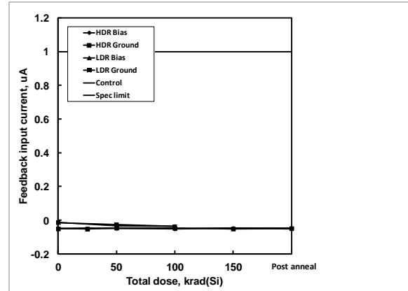
Figure 4: ISL75051SEH feedback pin input current as a function of biased and grounded high and low dose rate irradiation and subsequent high temperature accelerated post-high dose rate aging at 100^{\circ}\text{C} . The dose rate was 80 \text{ rad}(\text{Si})/\text{s} . Sample size was 6 for the high dose rate cells and 4 for the low dose rate cells, and three control units were used for the high dose rate test. The specification limits are -1.00\mu\text{A} - +1.00\mu\text{A} .
