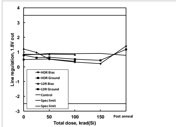
Figure 30: ISL75051SEH line regulation, 1.8V out, as a function of biased and grounded high and low dose rate irradiation and subsequent high temperature accelerated post-high dose rate aging at 100°C. The dose rate was 80 rad(Si)/s. Sample size was 6 for the high dose rate cells and 4 for the low dose rate cells, and three control units were used for the high dose rate test. The specification limits are -2.500mV to +3.500mV.
