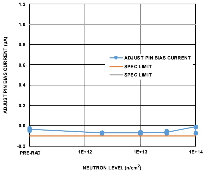
FIGURE 2. ISL75051SEH adjust ('feedback') pin bias current as a function of 1MeV equivalent neutron irradiation at 2 \times 10^{12} \text{ n/cm}^2 , 1 \times 10^{13} \text{ n/cm}^2 , 3 \times 10^{13} \text{ n/cm}^2 , and 1 \times 10^{14} \text{ n/cm}^2 . The plot shows the population median, minimum, and maximum at each downpoint. Sample size for each cell was five. The SMD limit is 1.0µA maximum; the -0.1µA bound is an ATE limit.
