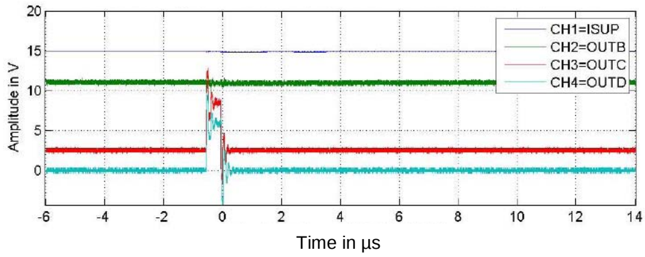
Figure 6: Short duration ( < 500 ns) low-high-low transients on OUTC and OUTD (Ag ions, \text{LET} = 86.4 \text{ MeV/mg/cm}^2 , V_{\text{IN}} = 6.1 \text{ V} , T_{\text{C}} = 125^\circ\text{C} )
