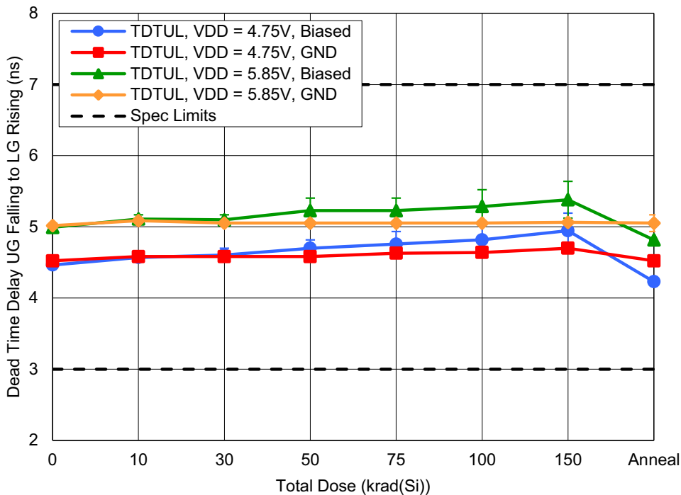
Figure 20. ISL73041SEH dead time delay, UG falling to LG rising ( t_{D\text{TUL}} ) with V_{DD} = 4.75\text{V} or 5.85\text{V} , and with R_{DU} = R_{DL} = 1\text{k}\Omega to GND as a function of HDR irradiation and anneal for biased and grounded configurations. The error bars (if visible) represent the minimum and maximum measured values. The datasheet limits are a minimum of 3ns and a maximum of 7ns.
