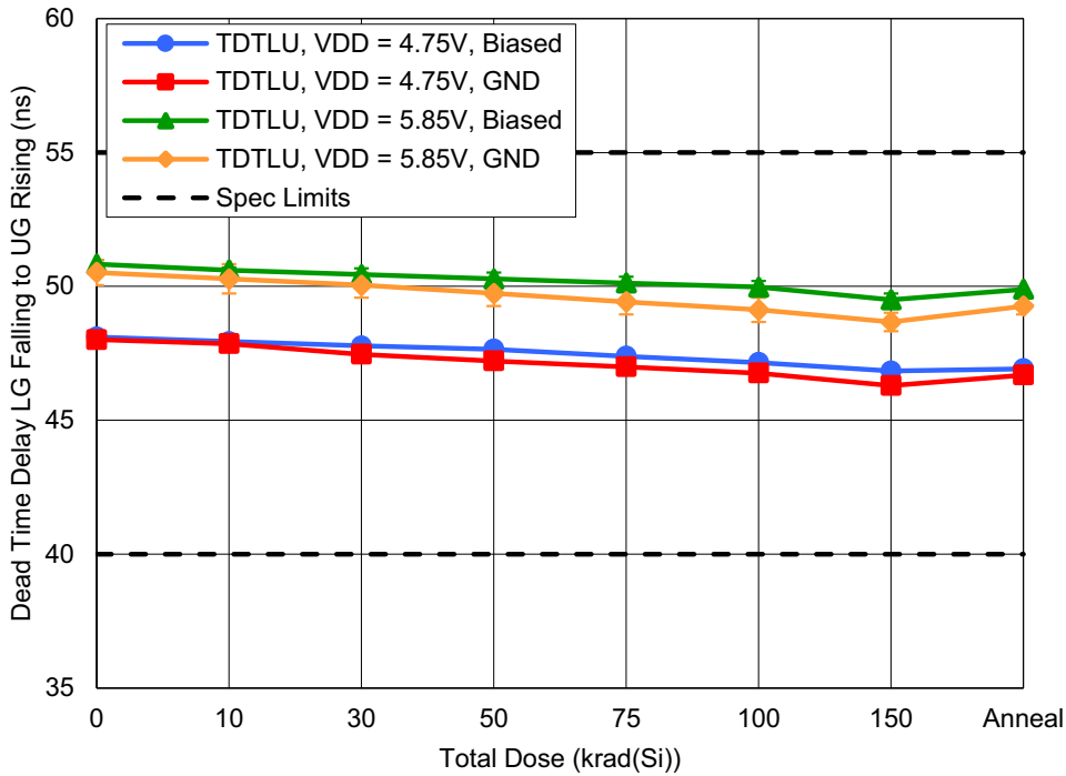
Figure 19. ISL73041SEH dead time delay, LG falling to UG rising ( t_{D\text{TLU}} ) with V_{DD} = 4.75\text{V} or 5.85\text{V} , and with R_{DU} = R_{DL} = 10\text{k}\Omega to GND as a function of HDR irradiation and anneal for biased and grounded configurations. The error bars (if visible) represent the minimum and maximum measured values. The datasheet limits are a minimum of 40ns and a maximum of 55ns.
