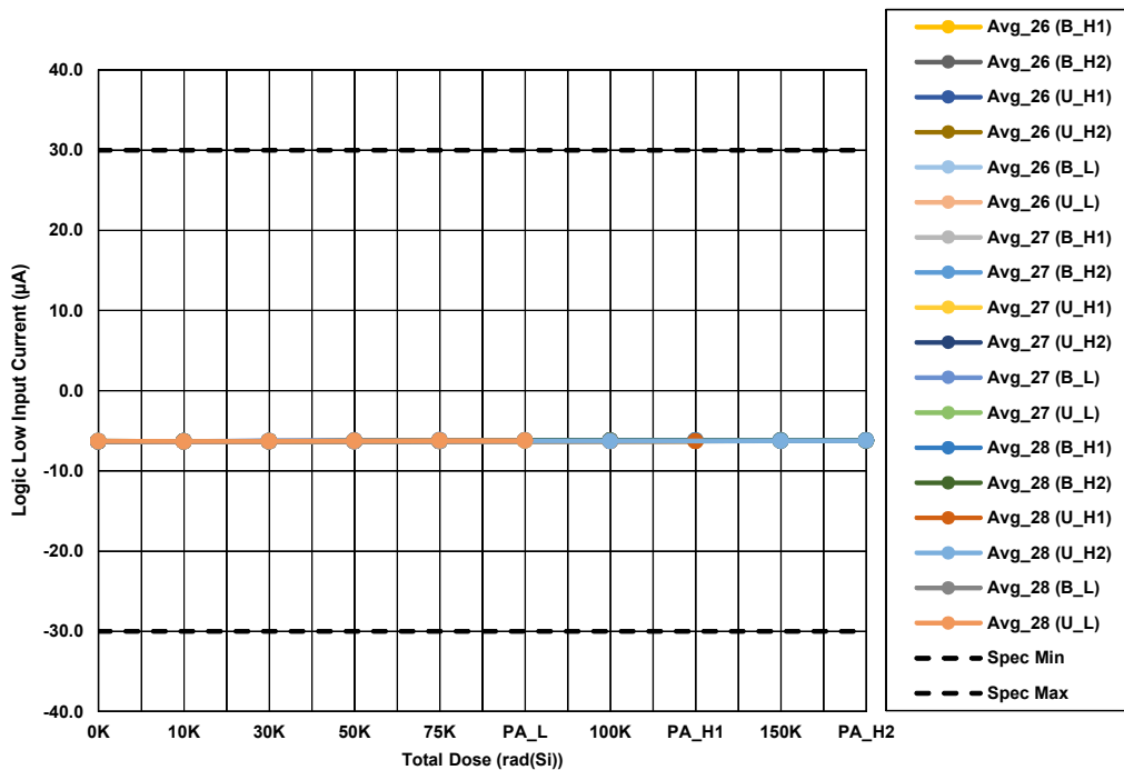
Figure 12. ISL72026CSEH, ISL72027CSEH, and ISL72028CSEH transmitter D input LOW ( I_{IL} ) for 3.0V supply, as a function of low and high dose rate irradiation for the biased (B_ - per Figure 4 ) and unbiased (U_ - all pins grounded) cases. The post-irradiation SMD limits are -30\mu\text{A} to +30\mu\text{A} .
