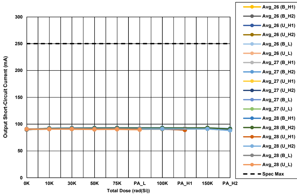
Figure 14. ISL72026CSEH and ISL72027CSEH transmitter output short-circuit current ( I_{O_{SC}} ) for 3.0V supply, V_{CANL} = 12V and V_{CANH} = open , as a function of low and high dose rate irradiation for the biased (B_ - per Figure 4 ) and unbiased (U_ - all pins grounded) cases. The post-irradiation SMD limit is 250mA maximum.
