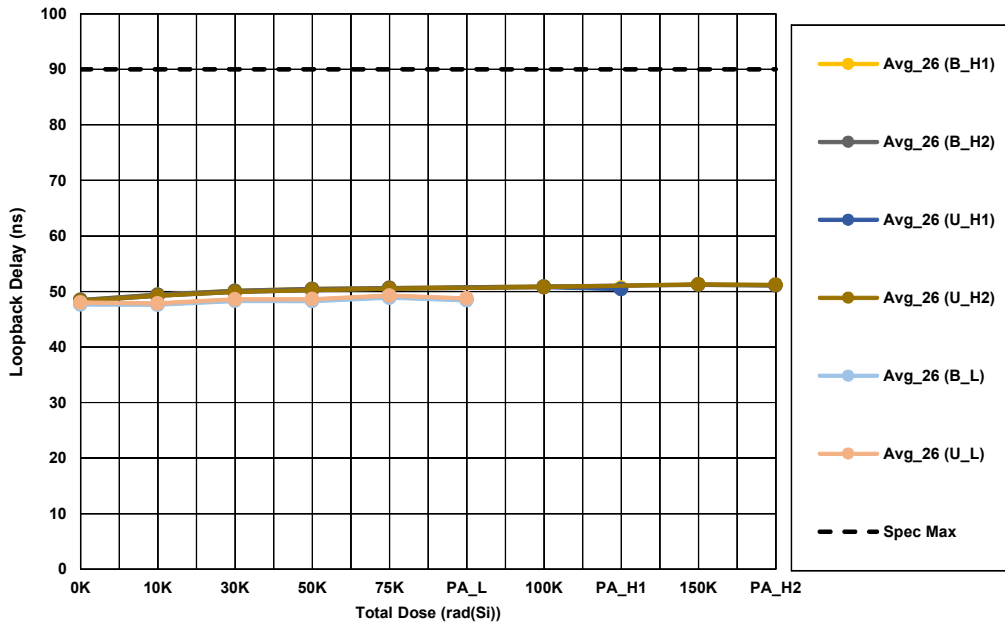
Figure 64. ISL72026CSEH loopback LOW to HIGH delay ( t_{LBK} ), for a 3.0V supply, IO to receiver output, as a function of low and high dose rate irradiation for the biased (B_ - per Figure 4) and unbiased (U_ - all pins grounded) cases. The post-irradiation SMD limit is 90ns maximum.
