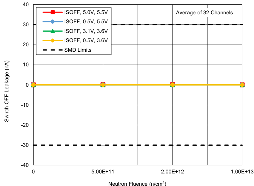
Figure 5. ISL71831SEH switch input OFF leakage average of all 32 channels with V^+ = 5.5V , V_{IN} = 5.0V , V_{OUT} = 0.5V , or V^+ = 5.5V , V_{IN} = 0.5V , V_{OUT} = 5.0V , or V^+ = 3.6V , V_{IN} = 3.1V , V_{OUT} = 0.5V , or V^+ = 3.6V , V_{IN} = 0.5V , V_{OUT} = 3.1V following irradiation to each level. The error bars (if visible) represent the minimum and maximum measured values across all channels. The post – TID irradiation SMD limits are a minimum of -30nA with a maximum of 30nA for both supply voltages.
