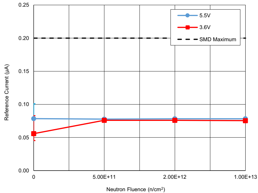
Figure 18. ISL71831SEH reference supply current with V^+ = V_{\text{REF}} = 5.5\text{V} and 3.6\text{V} following irradiation to each level. The error bars (if visible) represent the minimum and maximum measured values. The post - TID irradiation SMD limit is a maximum of 0.2\mu\text{A} for both voltages.
