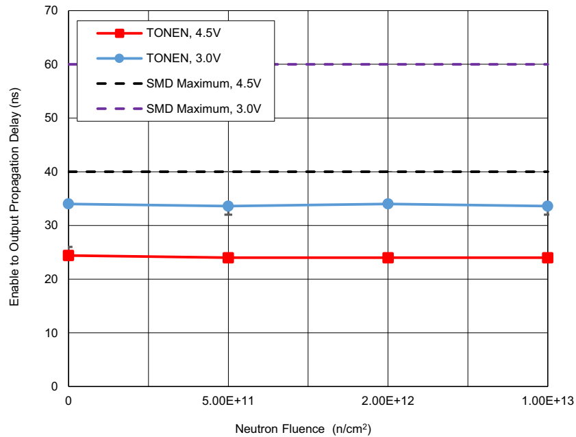
Figure 22. ISL71831SEH enable ON to multiplexer output propagation delay with V^+ = 4.5V and 3.0V following irradiation to each level. The error bars (if visible) represent the minimum and maximum measured values. The post – TID irradiation SMD limits are maximums of 40ns for a 4.5V supply voltage and 60ns for a 3.0V supply voltage.
