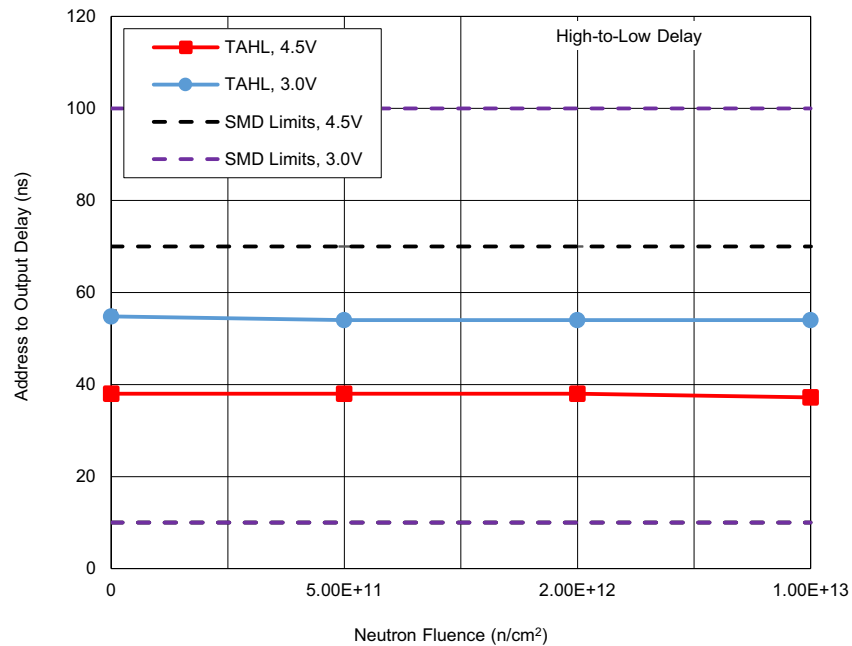
Figure 20. ISL71831SEH address input to multiplexer output delay (HIGH to LOW) with V^+ = 4.5V, 3.0V following irradiation to each level. The error bars (if visible) represent the minimum and maximum measured values. The post – TID irradiation SMD limits are a minimum of 10ns with a maximum of 70ns for a 4.5V supply voltage and a minimum of 10ns with a maximum of 100ns for a 3.0V supply voltage.
