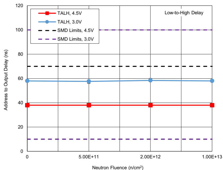
Figure 19. ISL71831SEH address input to multiplexer output delay (LOW to HIGH) with V^+ = 4.5\text{V} and 3.0\text{V} following irradiation to each level. The error bars (if visible) represent the minimum and maximum measured values. The post - TID irradiation SMD limits are a minimum of 10ns with a maximum of 70ns for a 4.5V supply voltage and a minimum of 10ns with a maximum of 100ns for a 3.0V supply voltage.
