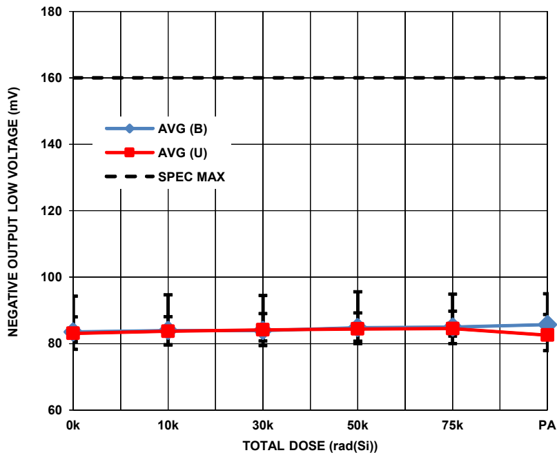
FIGURE 16. ISL70617SEH negative output LOW output voltage with I_{OUT} = 0mA at \pm 18V supplies as a function of low dose rate irradiation for the Biased (B) (per Figure 1) and Unbiased (U) (all pins grounded) cases. The error bars represent the minimum and maximum measured values. The post-irradiation SMD limit is 160mV maximum. The positive output LOW voltage (not shown) showed similar stability.
