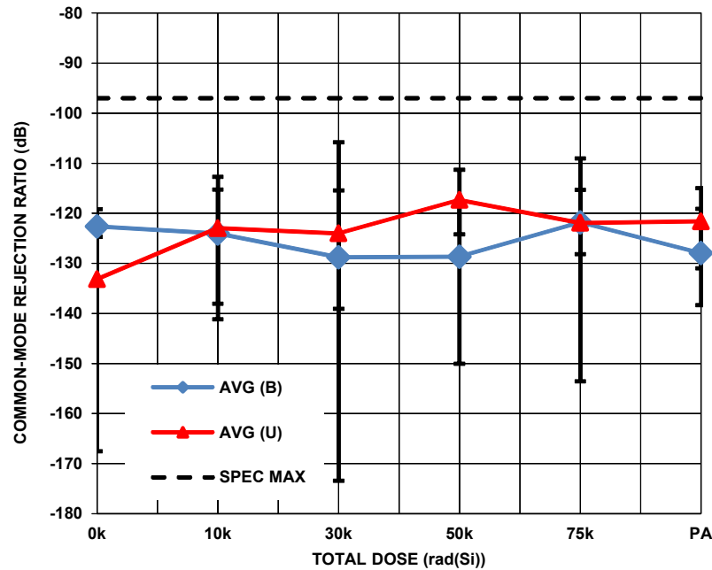
FIGURE 11. ISL70517SEH common-mode rejection ratio, \pm 15V supplies, gain of 1, as a function of low dose rate irradiation for the Biased (B) (per Figure 1) and Unbiased (U) (all pins grounded) cases. The error bars represent the minimum and maximum measured values. The post-irradiation SMD limit is -97dB maximum.
