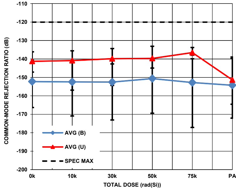
FIGURE 10. ISL70517SEH common-mode rejection ratio, \pm 15V supplies, gain of 100, as a function of low dose rate irradiation for the Biased (B) (per Figure 1) and Unbiased (U) (all pins grounded) cases. The error bars represent the minimum and maximum measured values. The post-irradiation SMD limit is -120dB maximum.
