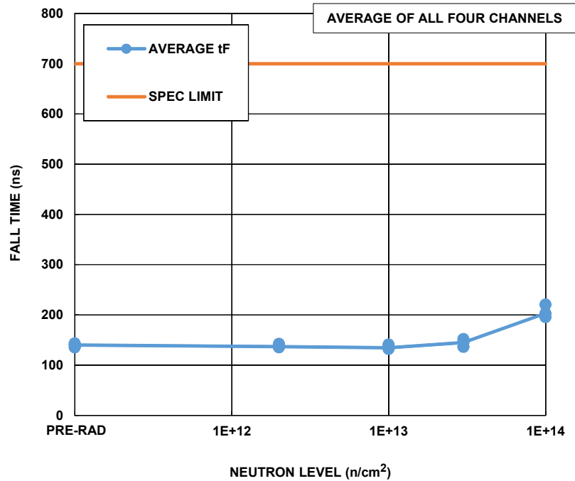
FIGURE 29. ISL70419SEH fall time, average of all four channels, as a function of 1MeV equivalent neutron irradiation at 2 \times 10^{12} \text{ n/cm}^2 , 1 \times 10^{13} \text{ n/cm}^2 , 3 \times 10^{13} \text{ n/cm}^2 , and 1 \times 10^{14} \text{ n/cm}^2 . The plot shows the population median, minimum, and maximum at each downpoint. Sample size for each cell was five. The post-total dose irradiation SMD limit is 700ns maximum.
