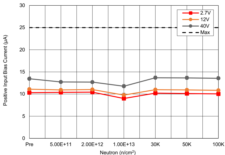
Figure 13. ISL7x100SEH positive input bias current ( I_{BIAS+} ) with V+ = V_{RS+} = 2.7V, 12V and 40V , V_{SEN} = 0mV , following irradiation to each level. The error bars (if visible) represent the minimum and maximum measured values. The post-irradiation SMD limit is 25\mu A maximum.
