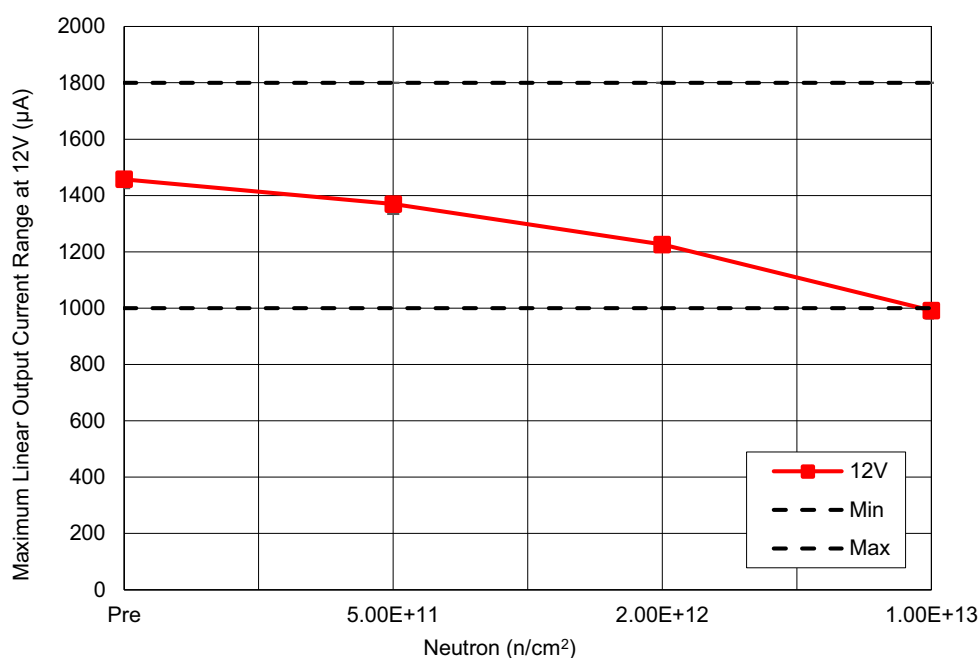
Figure 30. ISL7x100SEH maximum linear output current range ( I_{\text{OUT}} ) with V^+ = 12\text{V} and R_{\text{OUT}} = 0\Omega , following irradiation to each level. The error bars (if visible) represent the minimum and maximum measured values. The post-irradiation SMD limits are 1000 \mu\text{A} minimum and 1800 \mu\text{A} maximum.
