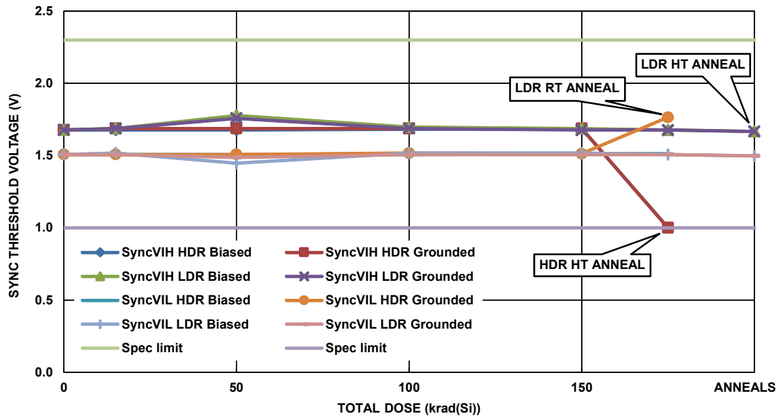
Figure 11. ISL70002SEH sync input HIGH and LOW threshold voltage, 5.5V supply, as a function of total dose irradiation at low and high dose rate for the unbiased (all pins grounded) and the biased (per Figure 2) cases. The low dose rate was 0.01rad(Si)/s and the high dose rate was 82.1rad(Si)/s. The high dose rate irradiations were followed by a high temperature biased anneal at 100°C for 168 hours. The low dose rate irradiations were followed by a 24-hour room temperature and a 168-hour 100°C anneal, both under bias. Sample size for the high dose rate cells was six for each cell, while the low dose rate cells were five samples each. The SMD limits are 2.3V maximum (HIGH) and 1V minimum (LOW).
