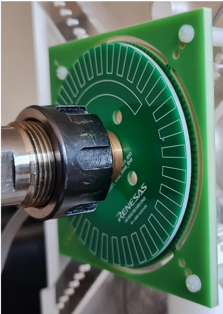
Figure 3. Setup
