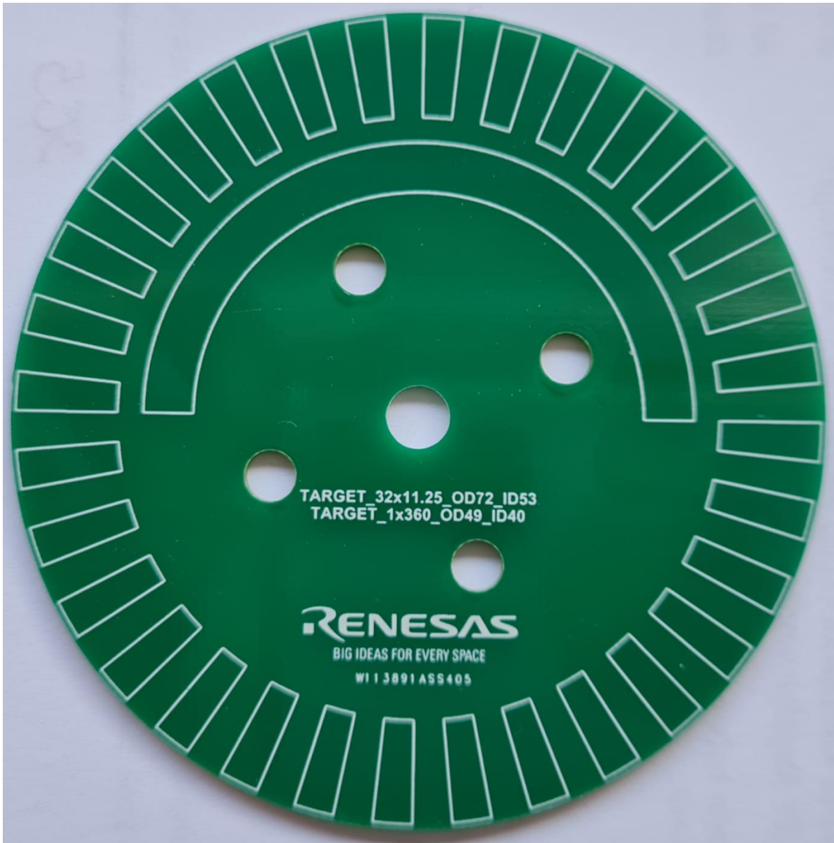
Figure 2. Sensor Target
