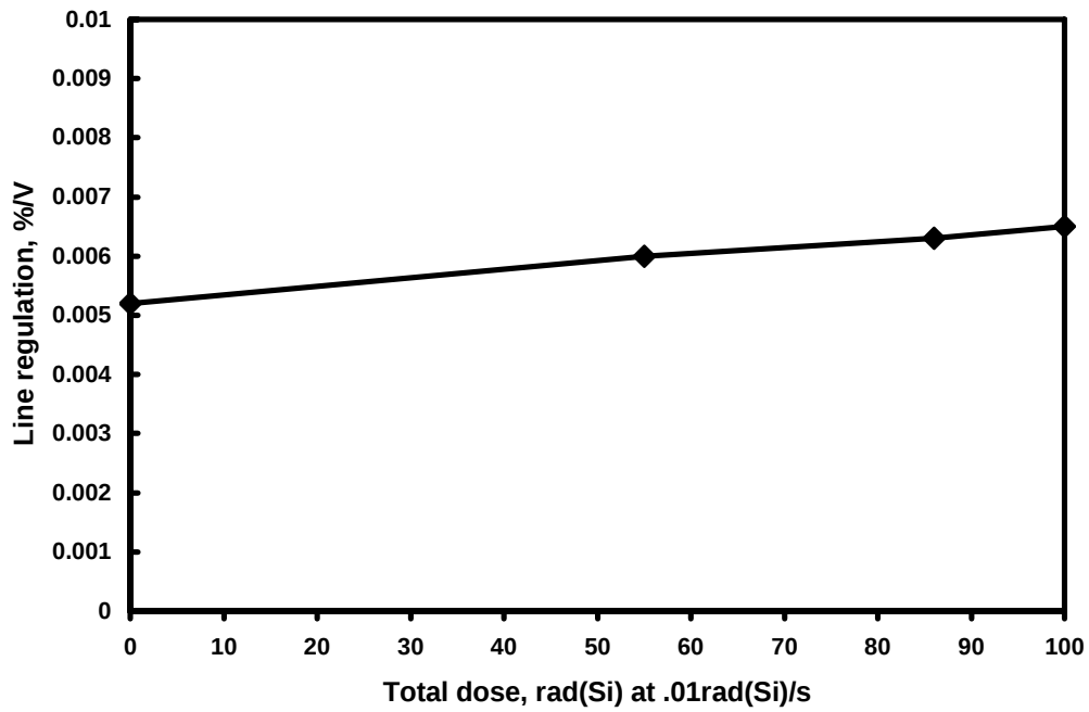
Figure 4: HS9S-117RH average line regulation as a function of total dose. Sample size was 12 parts. The maximum post-radiation line regulation specification is +/- .02%/V.
