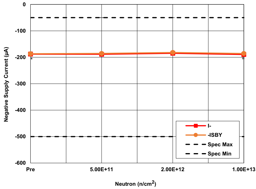
Figure 11. HS-1840AxH negative supply current (I-) and negative standby supply current (-I SBY ) following irradiation to each level. The error bars (if visible) represent the minimum and maximum measured values. The SMD limits are -500µA minimum and -50µA maximum.
