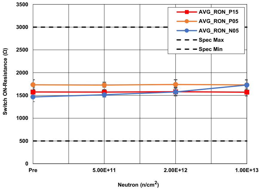
Figure 12. HS-1840AxH switch on-resistance (r DS(ON) ) following irradiation to each level. The error bars (if visible) represent the minimum and maximum measured values. The SMD limits are 500Ω minimum and 3000Ω maximum.
