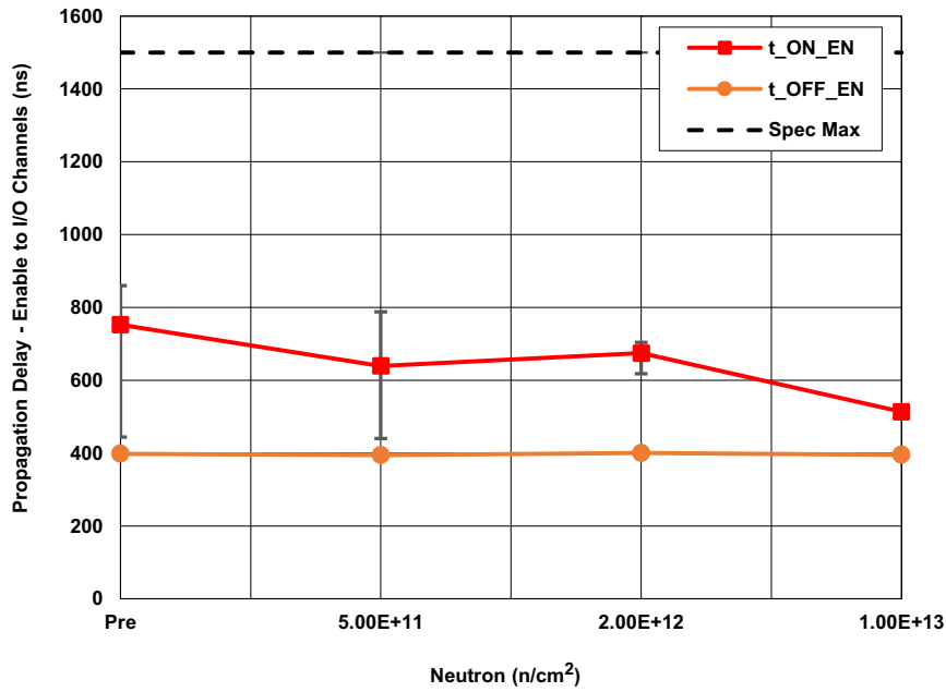
Figure 15. HS-1840AxH propagation delay time, enable to I/O channels (t on(EN) , t off(EN) ) following irradiation to each level. The error bars (if visible) represent the minimum and maximum measured values. The SMD limit is 1500ns maximum.
