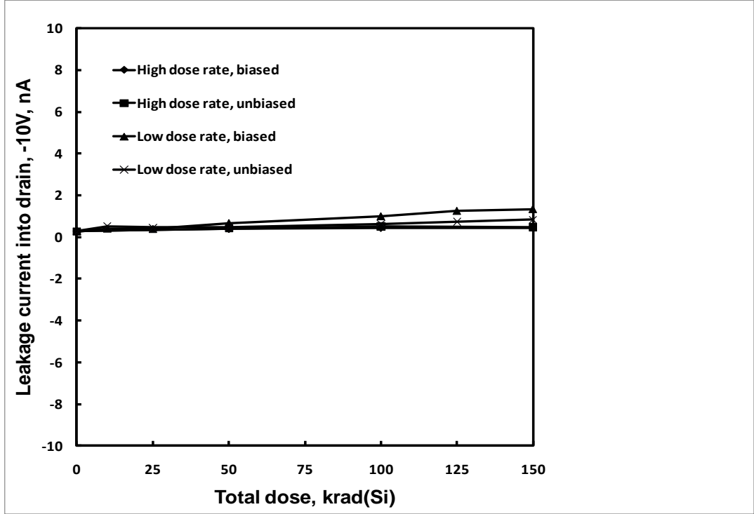
Figure 24: HS1840ARH leakage current into drain (-10V) as a function of total dose irradiation at low and high dose rate for the unbiased and biased cases. The post-irradiation SMD limits are -100 to 100nA.
