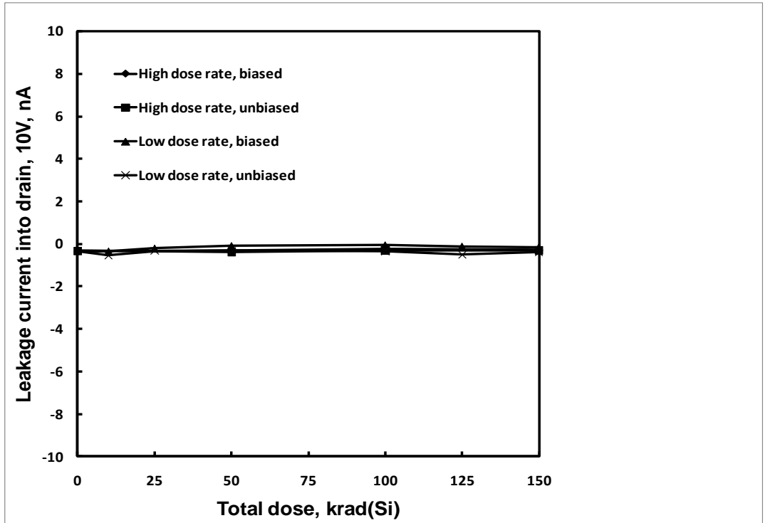
Figure 23: HS1840ARH leakage current into drain (10V) as a function of total dose irradiation at low and high dose rate for the unbiased and biased cases. The post-irradiation SMD limits are -100 to 100nA.
