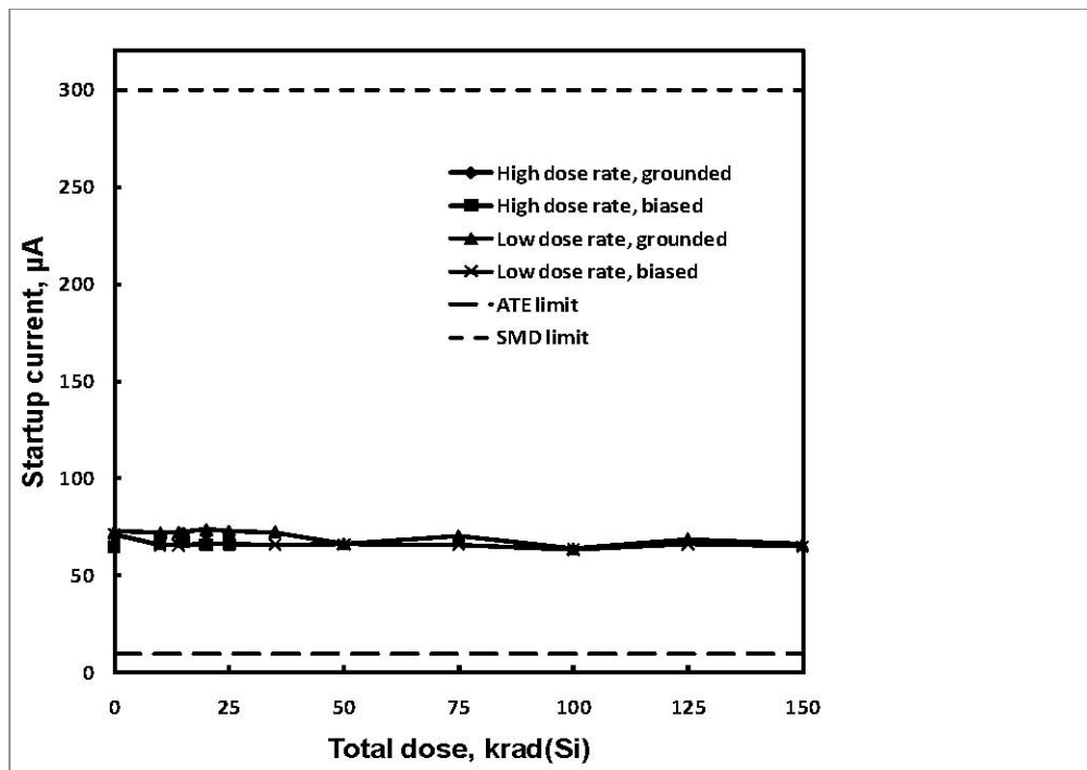
Fig. 50: IS-1825ASRH startup current as a function of total dose irradiation at low and high dose rate for the unbiased and biased cases. The post-irradiation SMD limit is 300µA maximum; the 10µA lower bound is an ATE limit.
