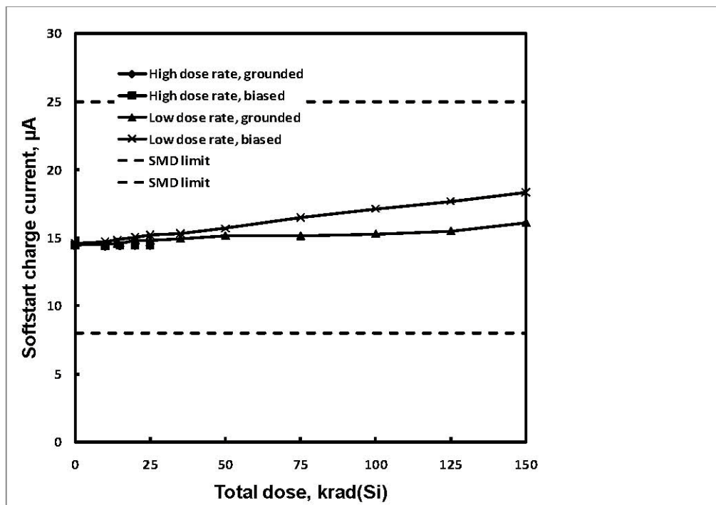
Fig. 31: IS-1825ASRH softstart charge current as a function of total dose irradiation at low and high dose rate for the unbiased and biased cases. The post-irradiation SMD limits are 8µA to 25µA.
