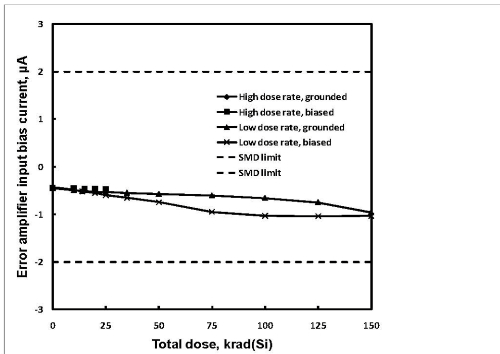
Fig. 18: IS-1825ASRH error amplifier input bias current as a function of total dose irradiation at low and high dose rate for the unbiased and biased cases. The post-irradiation SMD limits are -2µA to 2µA.
