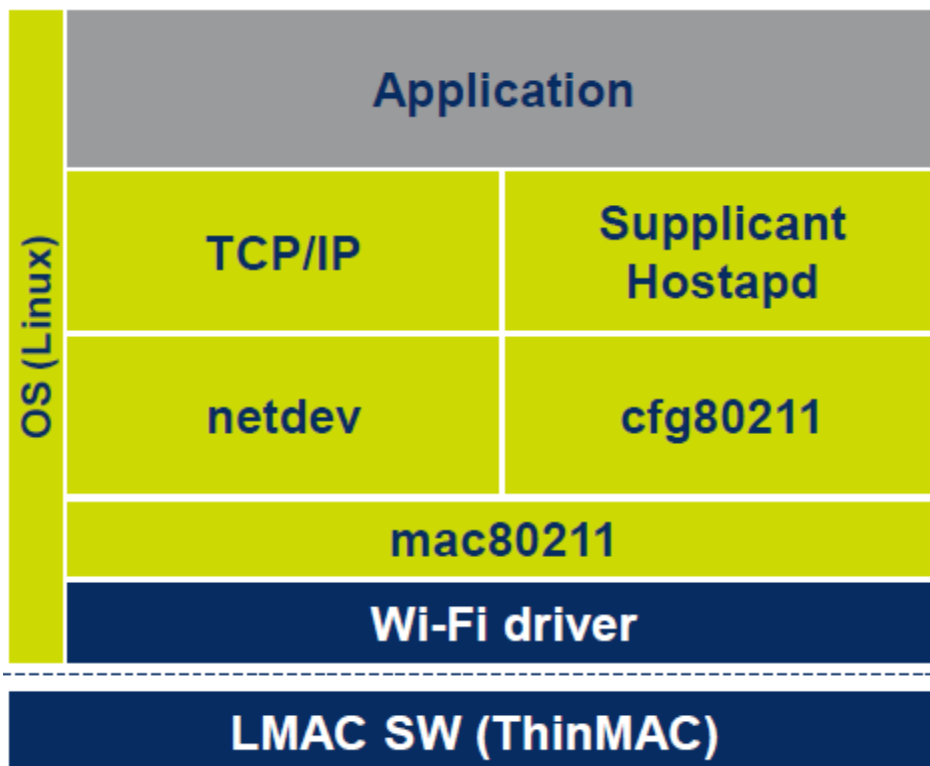
Figure 5: Linux Driver Architecture
