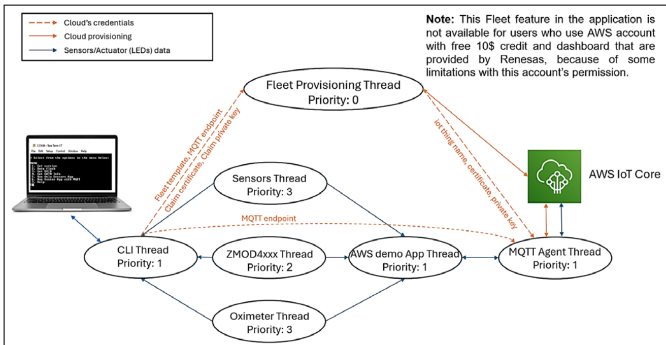
Figure 6. Thread Diagram when enabling Fleet feature
