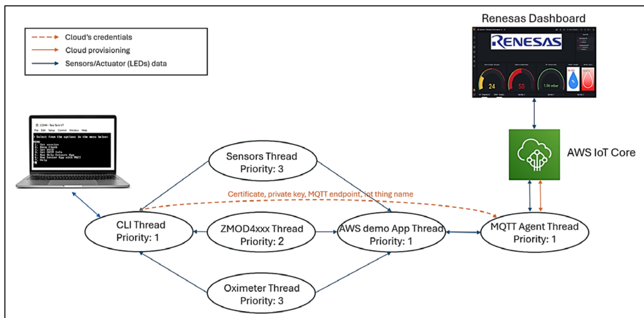
Figure 4. Thread Diagram
