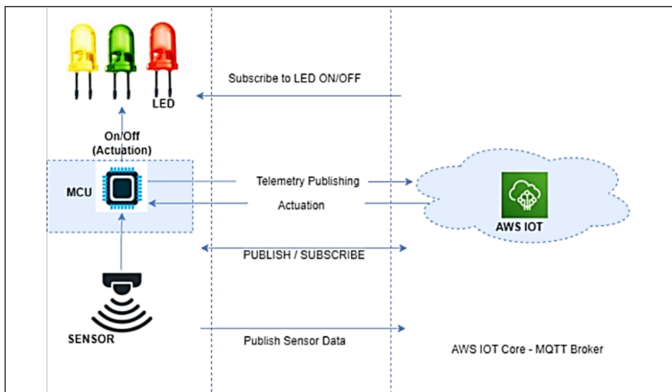
Figure 3. MQTT Publish/Subscribe to/from AWS IoT Core
