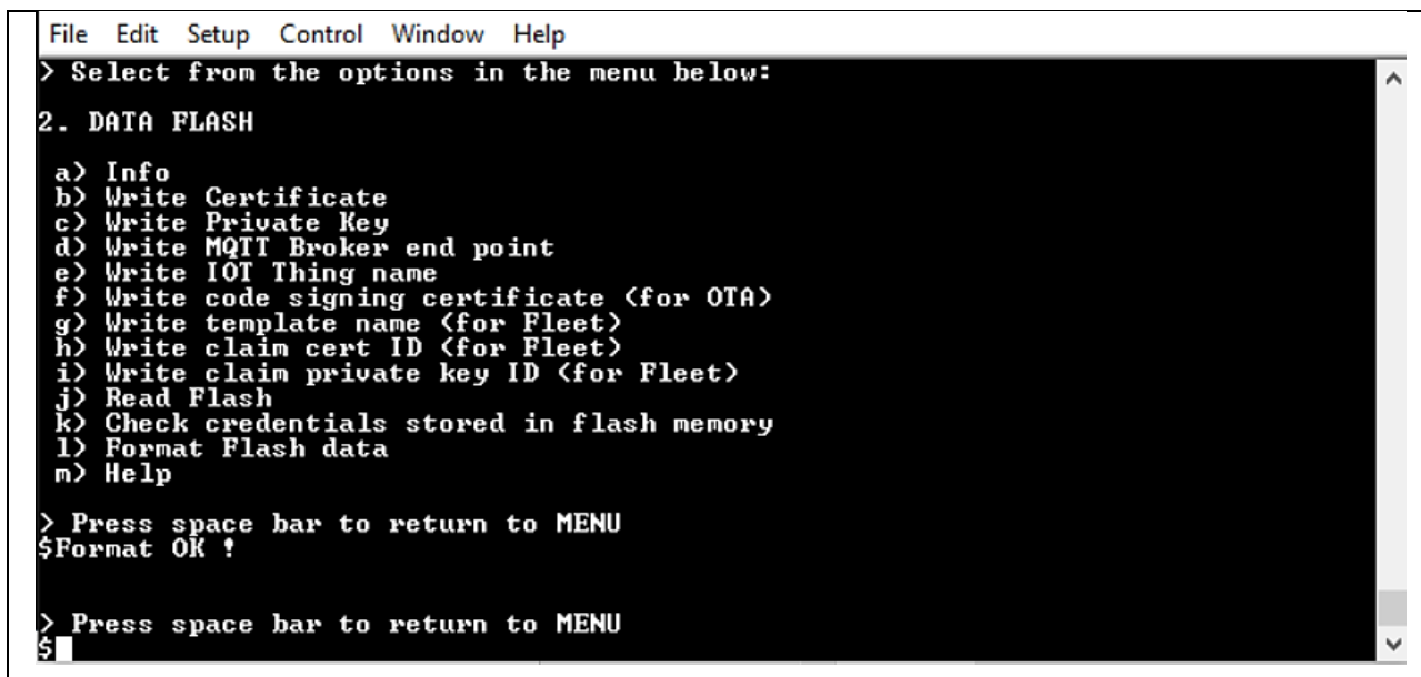
Figure 174. Save credentials for Fleet Provisioning (3/8)
